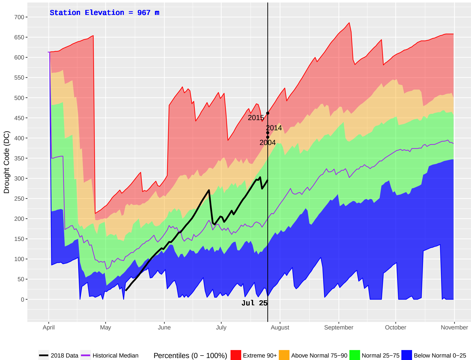
WONOWON (136) : Historical (1990–2016) and Current (2018) Noon Drought Code (DC)
